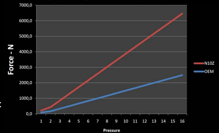
N10Z - Hydrostop System for Xplor Forks
